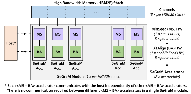
Figure 14: Overall system design of a SeGraM module. Our full design has four SeGraM modules and four HBM2E stacks.
