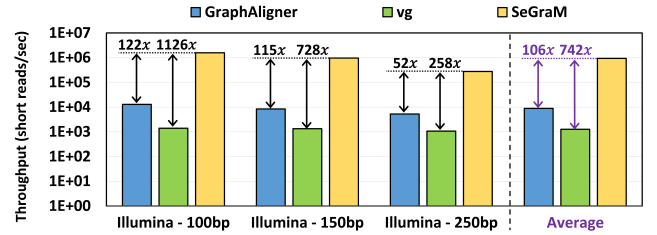
Figure 16: Throughput of GraphAligner, vg and SeGraM for short reads. 100/150/250bp stands for Illumina datasets with 100/150/250bp length reads.
