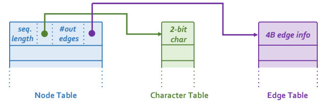
Figure 5: Memory layout of the graph-based reference.
