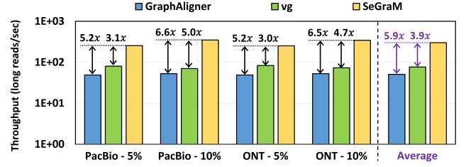
Figure 15: Throughput of GraphAligner, vg, and SeGraM for long reads. 5%/10% stands for PacBio/ONT datasets with 5%/10% read error rate.
