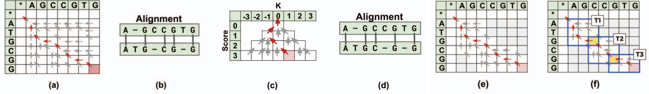
Fig. 2: Traceback matrices and alignments obtained from Needleman-Wunsch and WFA alignment algorithms, for example, input sequences R='AGCCGTG' and Q='ATGCGG' . (a) Traceback matrix for the Needleman-Wunsch algorithm with scoring parameters: \{\text{match}=2, \text{mismatch}=-1, \text{gap}=-1\} . Each cell stores a single traceback pointer pointing up, left, or diagonal, with the traceback path starting from the pink cell highlighted in red. (b) Alignment corresponding to the traceback path in (a). (c) Traceback matrix for the WFA algorithm with scoring parameters: \{\text{mismatch}=1, \text{gap}=1\} , with the traceback path starting from the pink cell highlighted in red. (d) Alignment corresponding to the traceback path in (c). (e) Traceback matrix for the X-Drop algorithm (adaptive banding) with scoring parameters same as (a) and \{x=3\} . Pruned cells are highlighted in gray, and the traceback path starting from the pink cell is highlighted in red. (f) Illustration of the tiling heuristic (GACT) with parameters: \{T=3, O=1\} . Overlapping cells between two consecutive tiles are highlighted in yellow, and the traceback path starting from the pink cell is highlighted in red.
