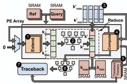
Fig. 8: TALCO-WFAA hardware design
