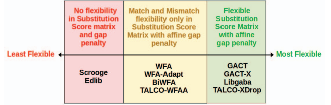
Fig. 9: Illustration of flexibility in the alignment scoring function of all evaluated tools, including TALCO. Tools with greater scoring flexibility tend to exhibit lower speed and memory efficiency but solve a more generalized formulation of the alignment problem with broader bioinformatic utility.
